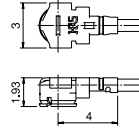
Form of Plug After Cable Wiring
